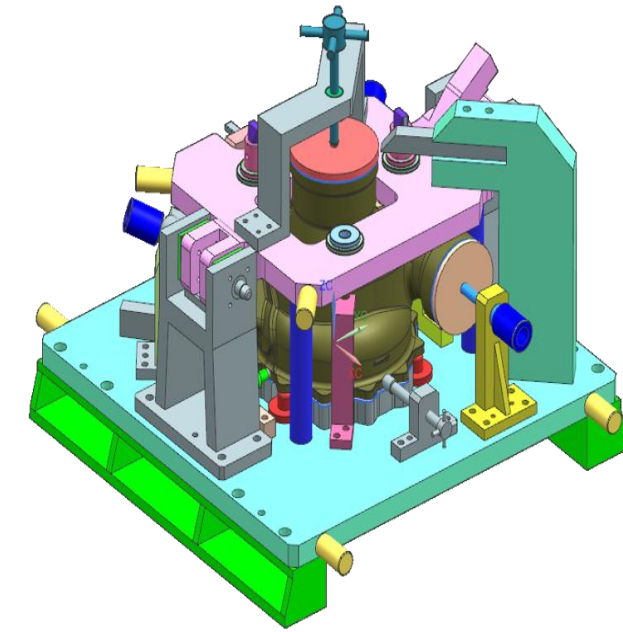
Jig & Fixture
